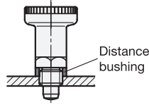
Indexing plungers GN 607 / GN 607.1
